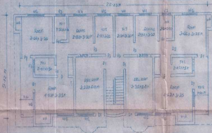
G.F. Plan
